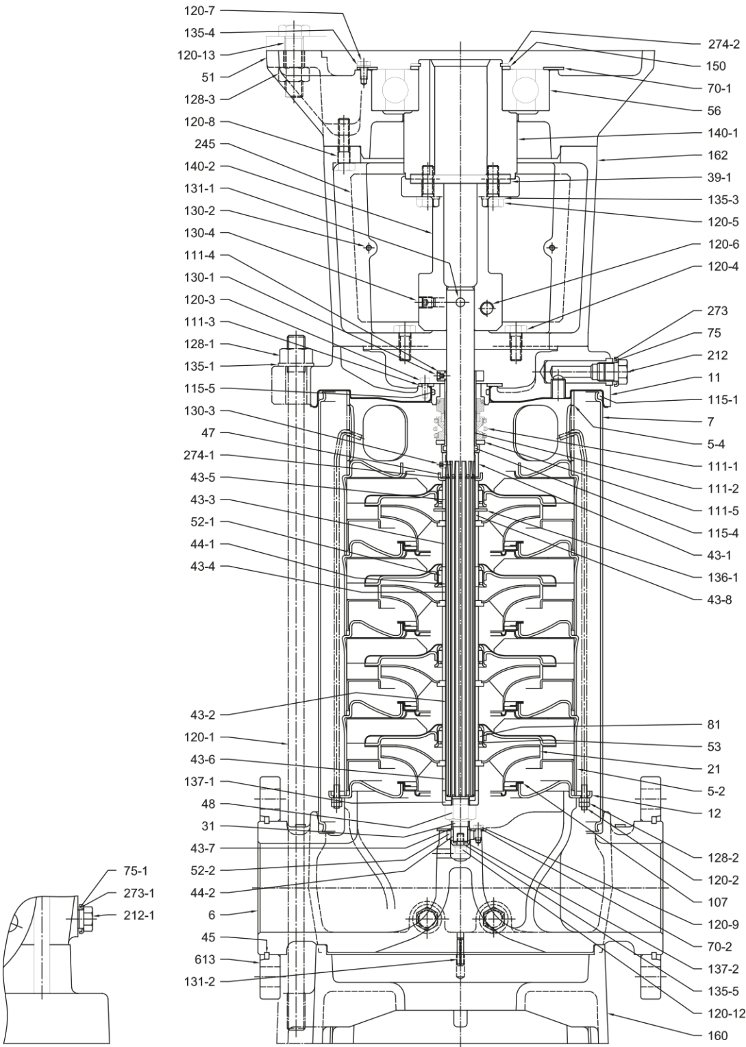
Pump with single ball bearing
